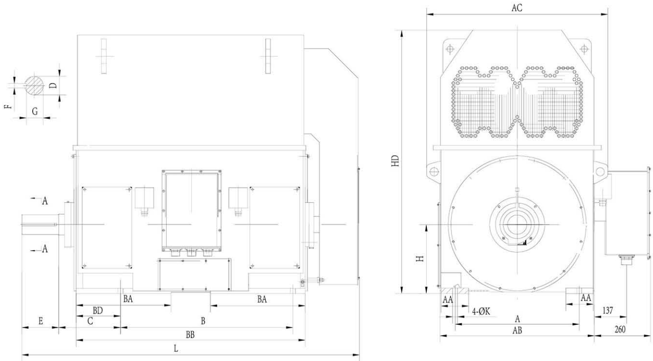
MOUNTING AND OVERALL DIMENSIONS OF YKK SERIES HIGH-VOLTAGE 3-PHASE INDUCTION MOTORS (6kV)
